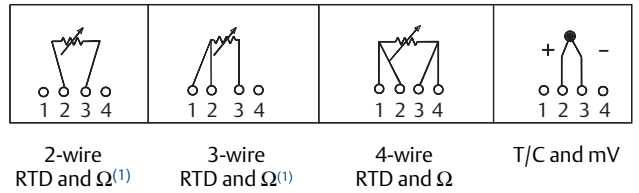
Figure 3. 248 Wireless Sensor Connection
