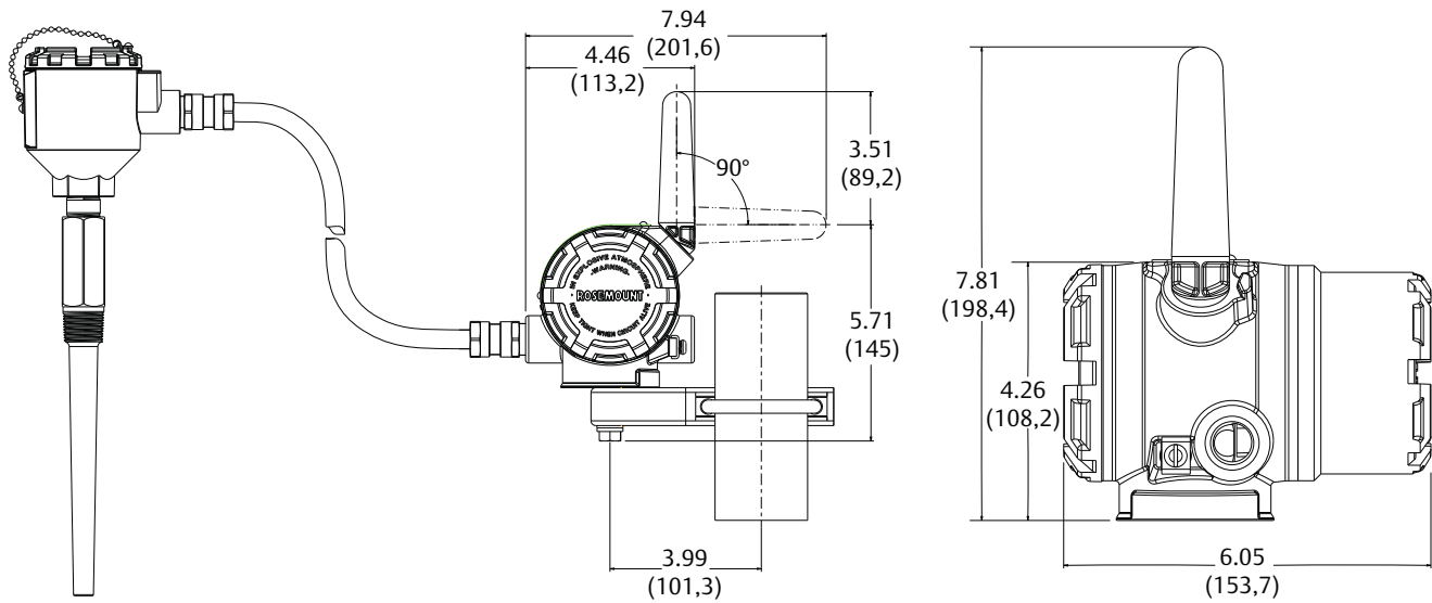
Figure 6. Rosemount 248 Wireless Remote Mount (Aluminum Housing)
