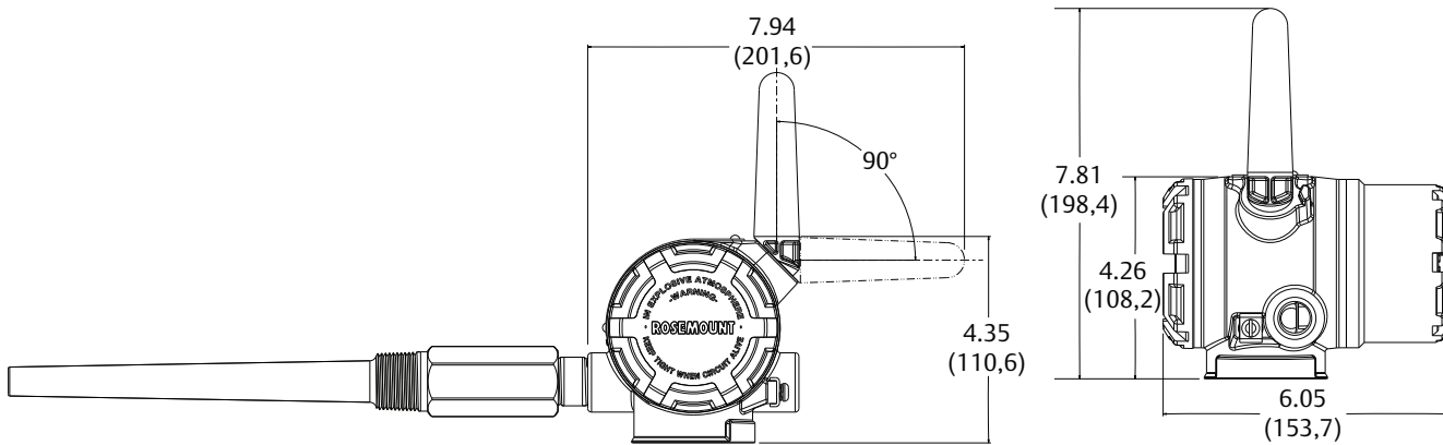
Figure 7. Rosemount 248 Wireless Direct Mount (Aluminum Housing)
