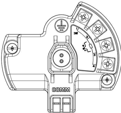
Figure 2. Rosemount 248 Wireless Sensor Terminal Block (Aluminum Housing)
