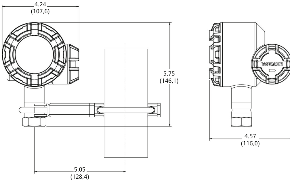
Figure 4. Rosemount 248 Wireless Remote Mount (Polymer Housing)
