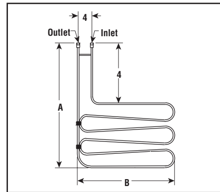
US4 — Dimensions (Inches)
