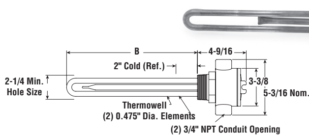
E4TP — Dimensions (Inches)
