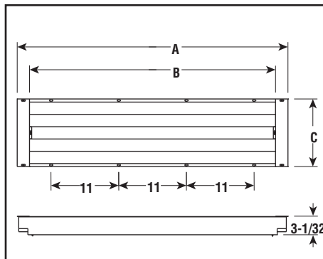
LC-4 — Dimensions (Inches)
