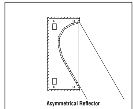
LC-4 — Asymmetrical Dim. (In)
