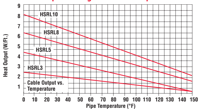
Thermal Output Ratings on Plastic Pipe with Aluminum Tape
