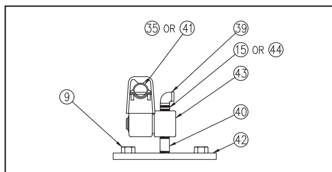
Figure B2 - Open Loop Cooling
