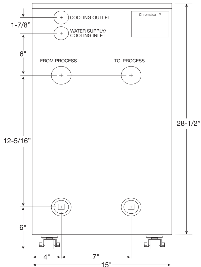
Rear View
