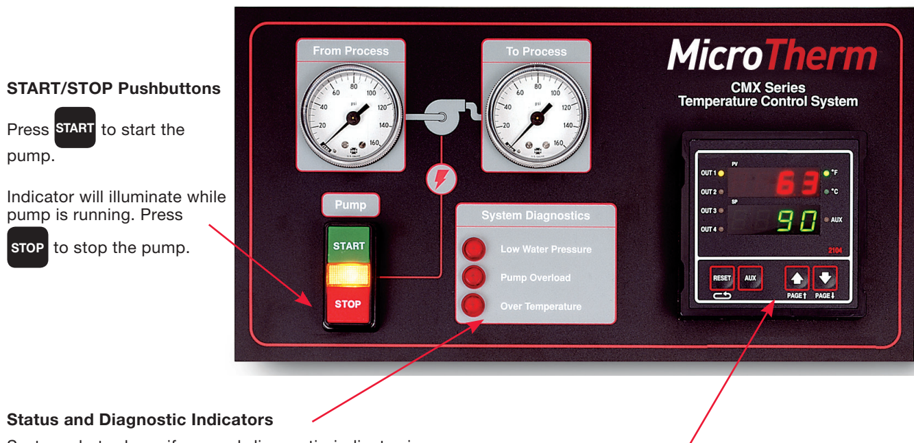
Figure 3.1 Control Panel Layout
