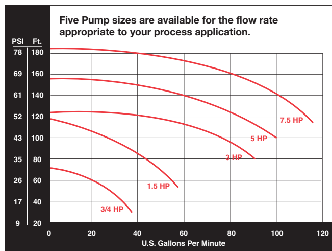
Pump Capacity
