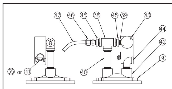
Figure B1 - Closed Loop Cooling
