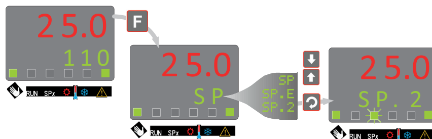
Example (switching from internal setpoint to SP.2)
