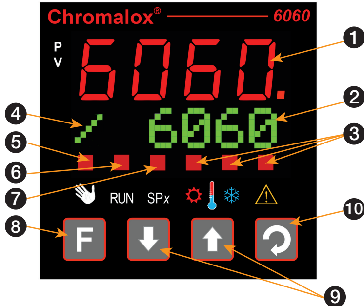
Fig. 5: Front View
