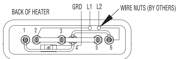
Single Phase Wiring
