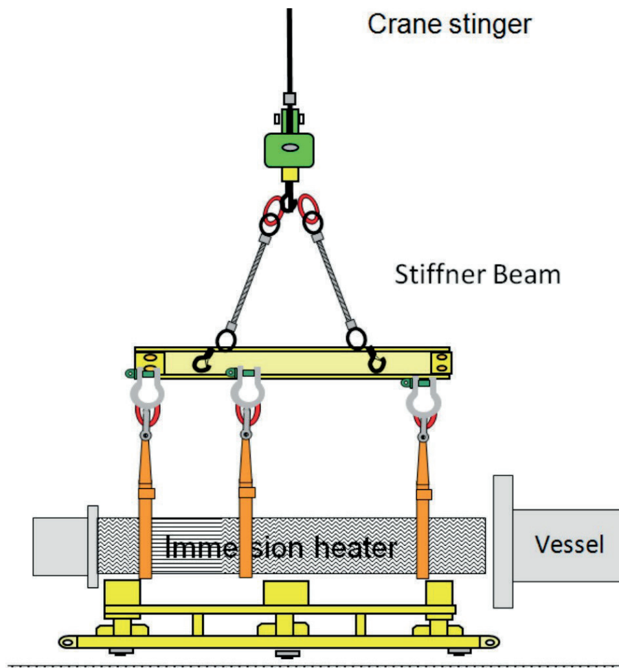
Figure C.1: Example removal procedure (for reference only)
