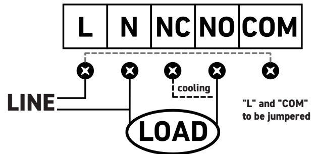
Wiring when load exceeds t'stat rating, pilot duty
