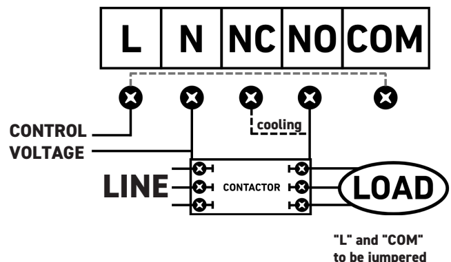
Wiring when load exceeds t'stat rating, pilot duty
